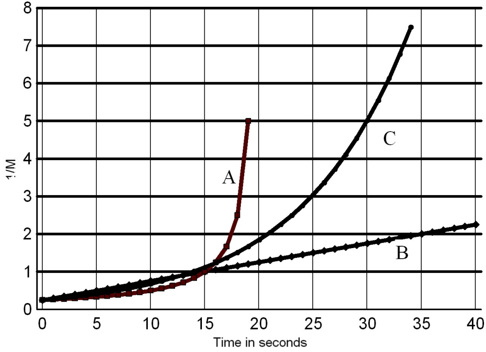
1/M vs. time
