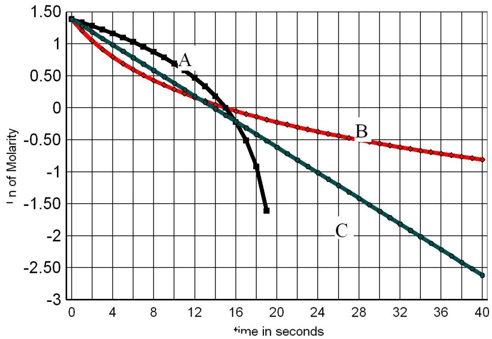
Ln of Molarity vs time
