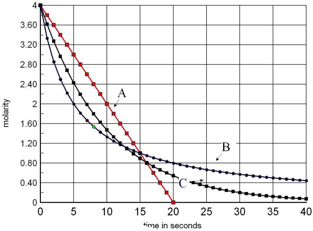
Concentration vs. time
